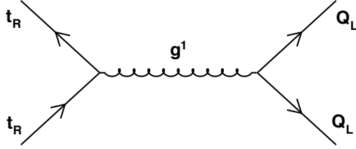
Figure 4: Feynman diagram showing how g^1 mediates a 4-top interaction at low energies.
