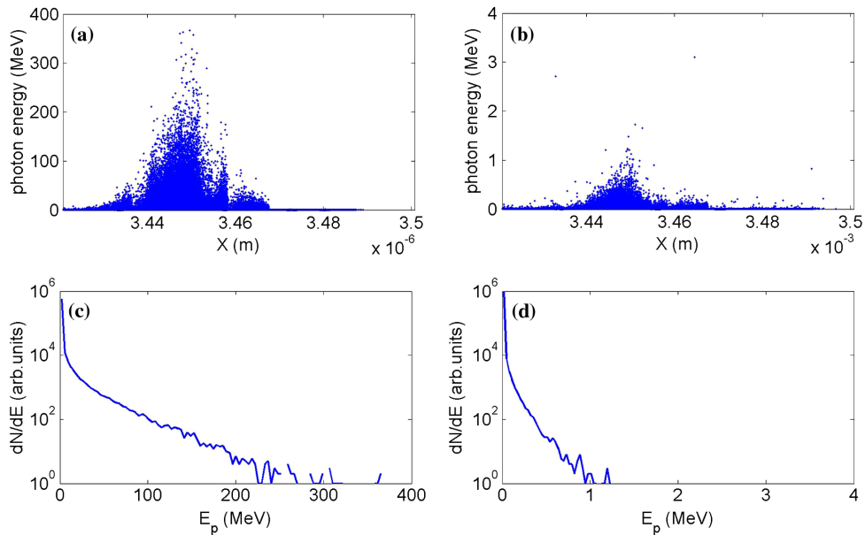
FIG. 6. The energy spectrum and spatial distribution of photon emitted from the wakefield driven by x-ray laser and optical one. (a) and (b) Photon energy distributions and (c) and (d) photon energy spectrum in the (a) and (c) x-ray driven case and (b) and (d) 1 eV optical laser driven case in a tube. The parameters are the same as in Fig. 5.
