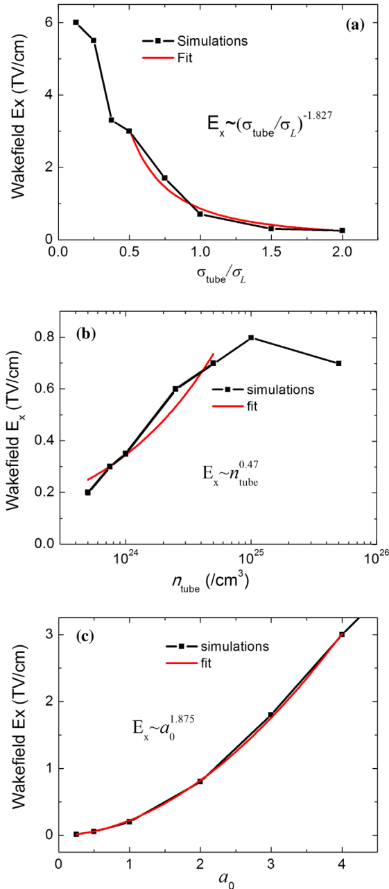
FIG. 7. Wakefield scalings in the x-ray regime with (a) tube radius, (b) tube wall density when the tube radius is fixed \sigma_{\text{tube}}/\sigma_L = 1 , and (c) laser intensity when the tube radius is fixed \sigma_{\text{tube}}/\sigma_L = 0.5 .
