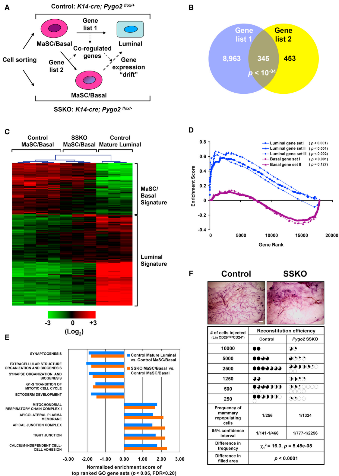
Figure 3. Transcriptional Profiling of Control and Pygo2 SSKO Mammary Populations
