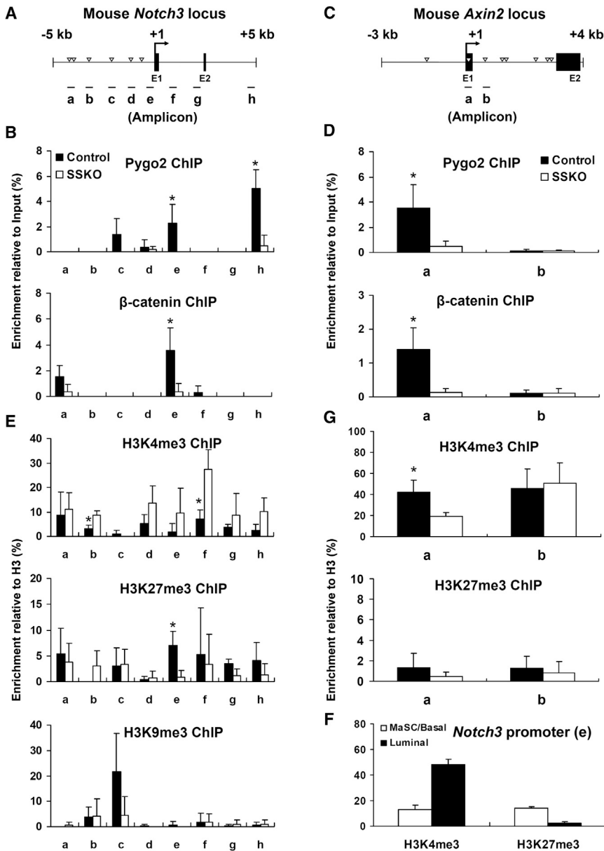
Figure 6. Pygo2 Regulates \beta -Catenin Binding and Chromatin Configuration at the Notch3 Locus
